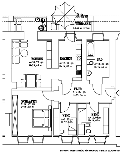
WE 1.2 WF=113,30qm
